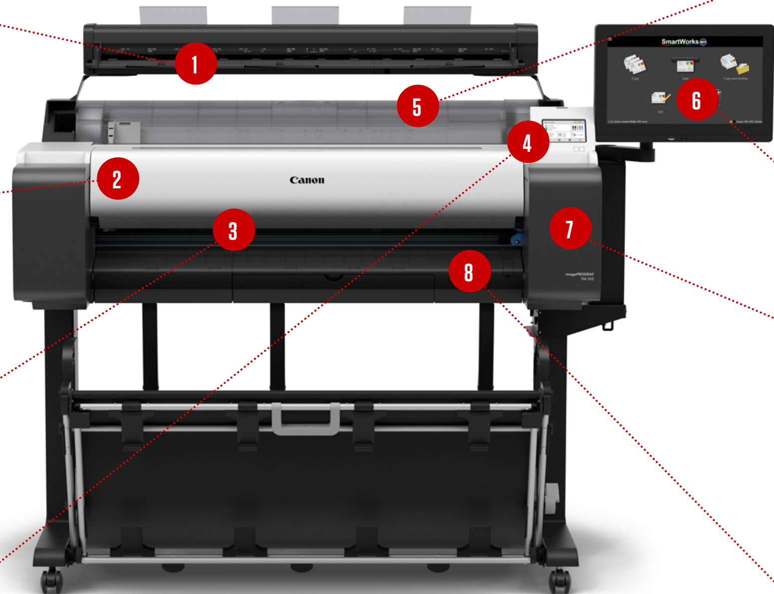
imagePROGRAF TM-355 MFP Z36
